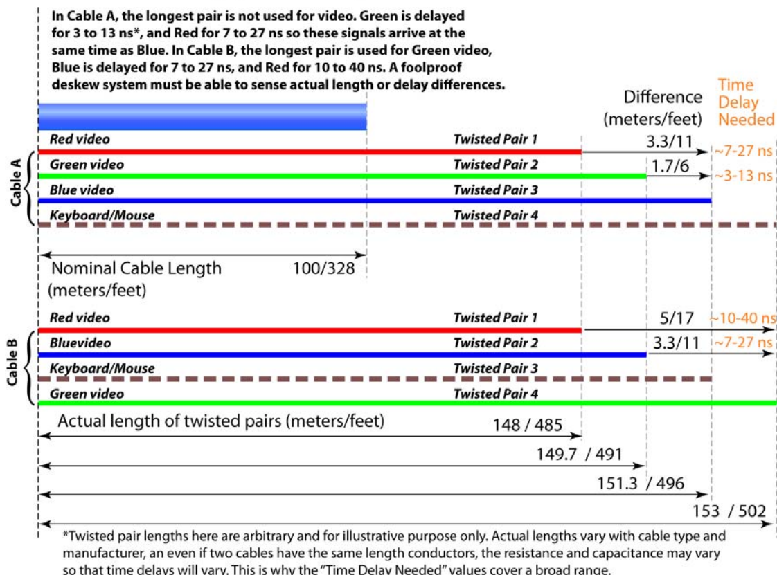
Figure 3. Using delay to slow earlier-arriving signals so they align with the latest-arriving signal.
